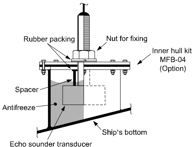
Figure 5.7 Inner-Hull installation
