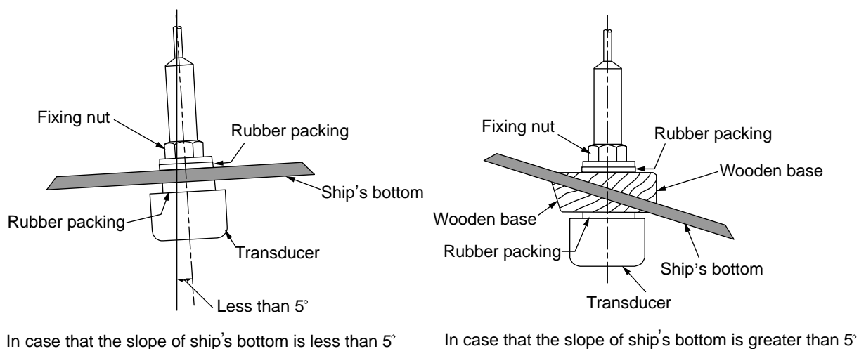
Figure 5.8 Through-hull Installation
